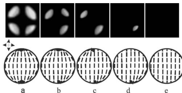
Figure 4. Dynamics of the spontaneous structural transition in the 5CB nematic droplet with a size of 15\ \mu\text{m} . The sample was prepared upon phase separation in the magnetic field H = 4\ \text{kOe} . During the formation, the droplet axis approximately coincided with the field direction. The directions of the polarizers are indicated by double arrows.
