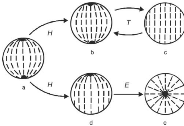
Figure 6. Schematic of the structural transition in the nematic droplets formed in magnetic field H : (a) bipolar structure, (b) bipolar configuration with broadened boojums, (c) homogeneous structure, (d) monopolar configuration, and (e) radial structure. T is a temperature of the cyclic transition. E is an electric field caused by flexoelectric polarization.
