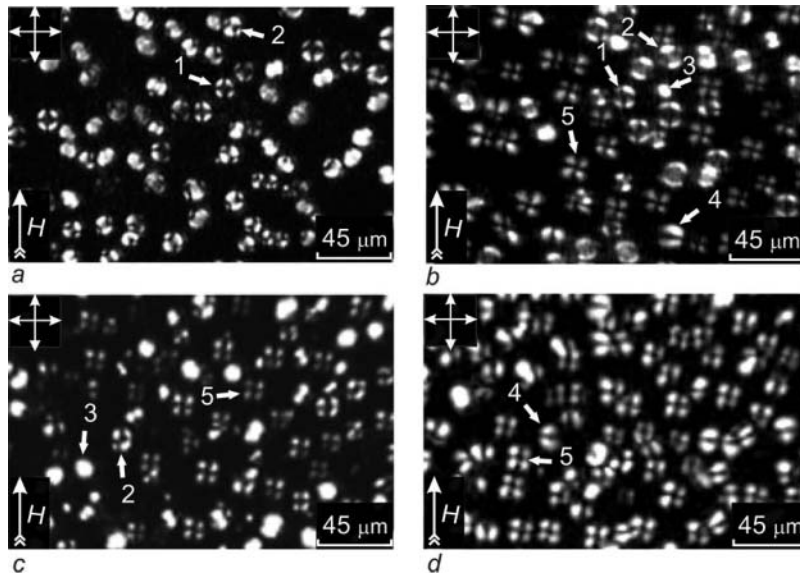
Figure 1. Ensemble of 5CB nematic droplets prepared at the temperature t = 24^\circ\text{C} in orienting magnetic field H : (a) H = 3 kOe, (b) H = 4 kOe, (c) H = 6 kOe, and (d) H = 15 kOe.
